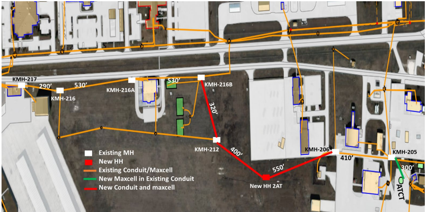
8.3 Figure 3: Fiber Optic Cable Route from ITB 1050 to EB ATCT.
