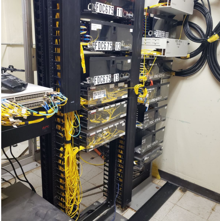
675 Equipment Rack
